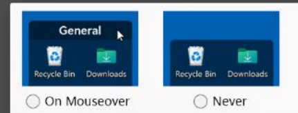
Customize Headers
